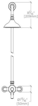
FRONT VIEW SCALE: 1"=1'-0"
