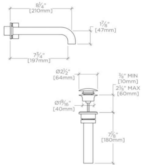
SIDE VIEW SCALE: 1\frac{1}{2}"=1'-0"
