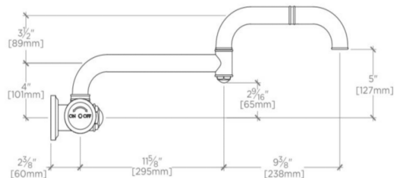
SIDE VIEW SCALE: 1\frac{1}{2}"=1'-0"
