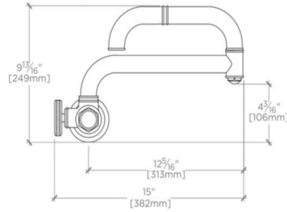
FOLDED VIEW SCALE: 1\frac{1}{2}"=1'-0"
