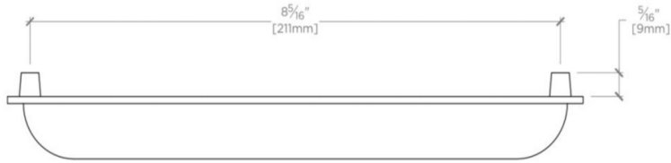
TOP VIEW
