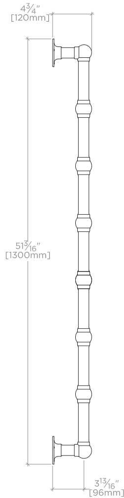
SIDE VIEW
